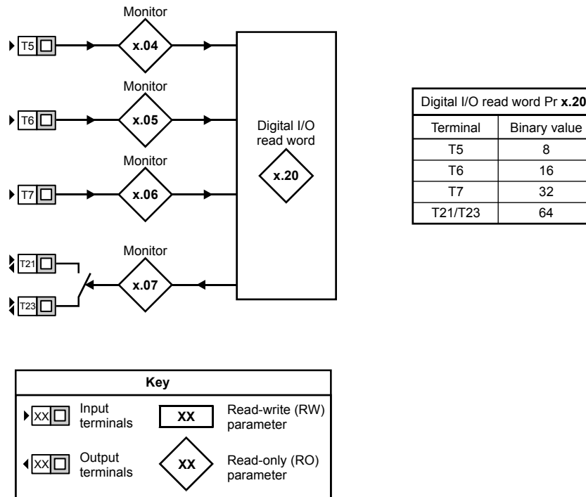
Figure 10-47 Menu 15D logic diagram*
