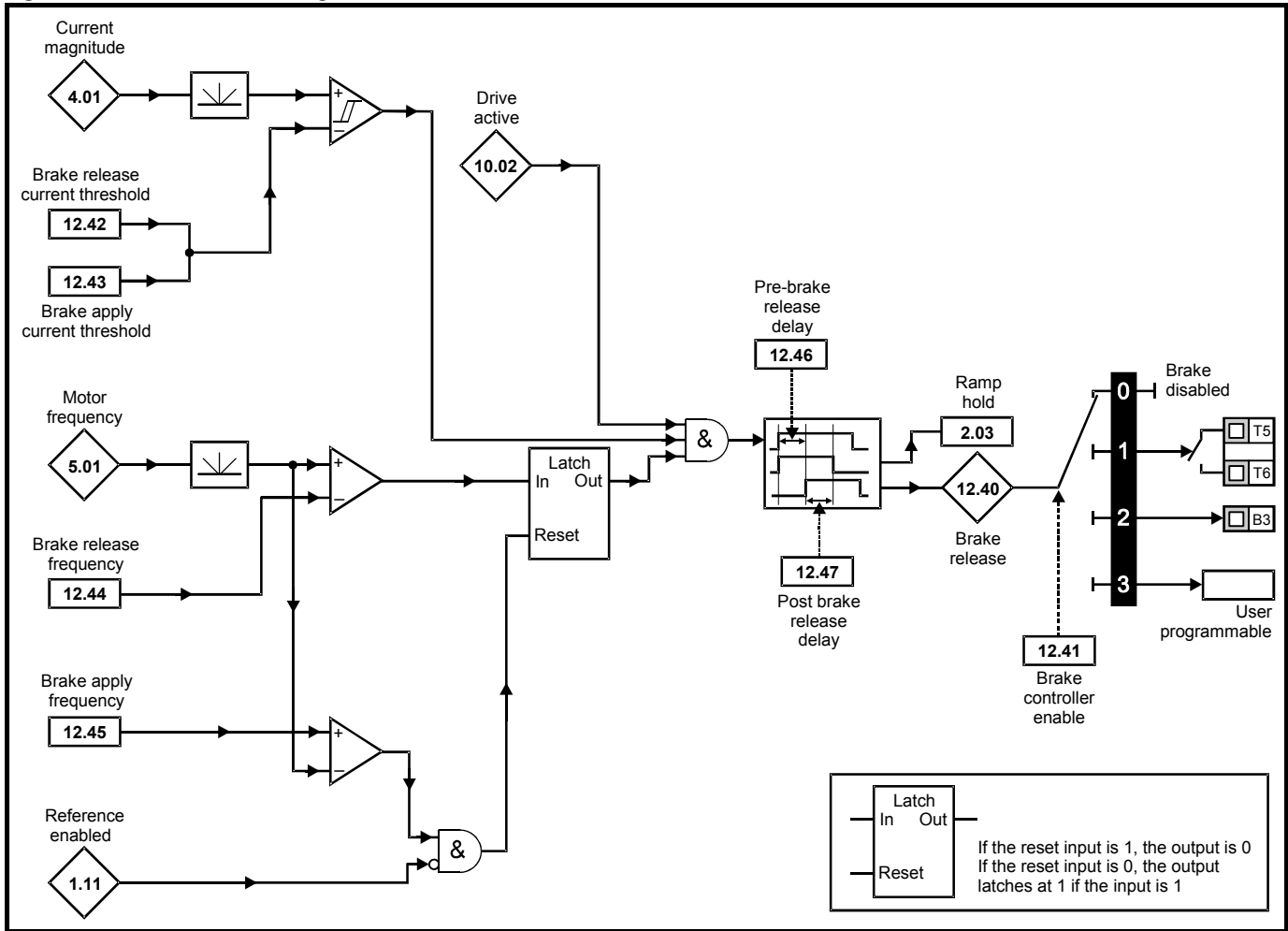
Figure 10-41 Brake sequence
